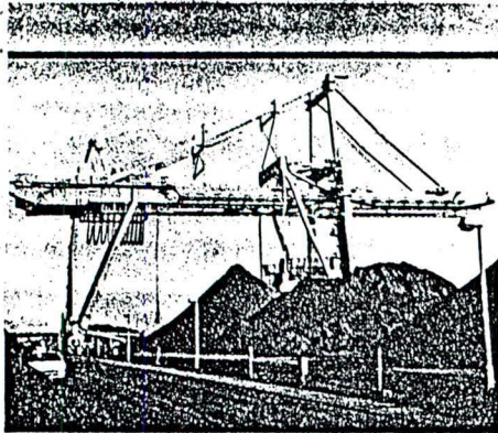
MAN GHH was awarded the contract to deliver a new 85 tonnes lift capacity grab unloader to EMO, Rotterdam in January 1990. Checked and approved for safety in March this year the unloader was put into operation last month (April) and offers maximum handling rates of 5100tph in ore and 4200tph in coal. (see main article)
